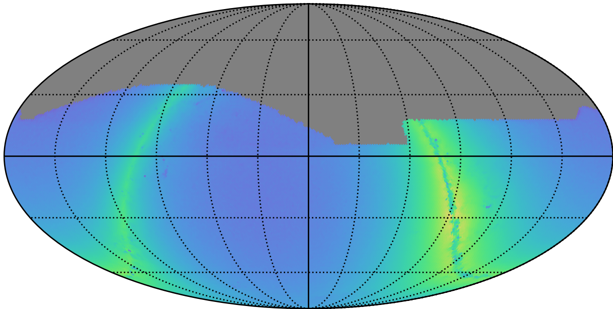
too_elab_heavy_r32_d2_griz_v3.4_10yrs i: Nstars_no_crowding
