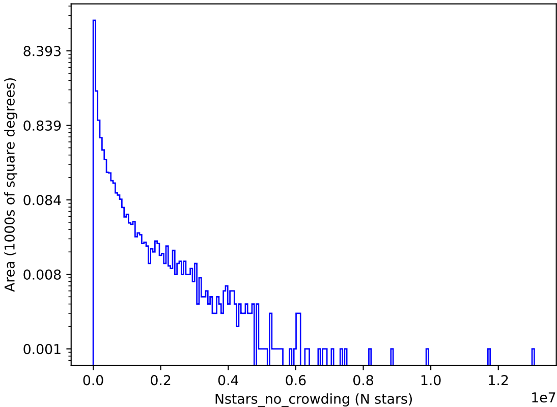
too_elab_heavy_r32_d2_griz_v3.4_10yrs g: Nstars_no_crowding
