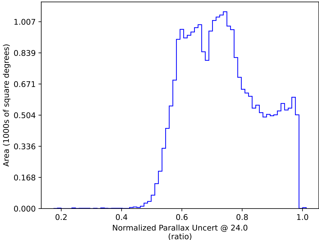
too_elab_heavy_r32_d2_griz_v3.4_10yrs : Normalized Parallax Uncert @ 24.0
