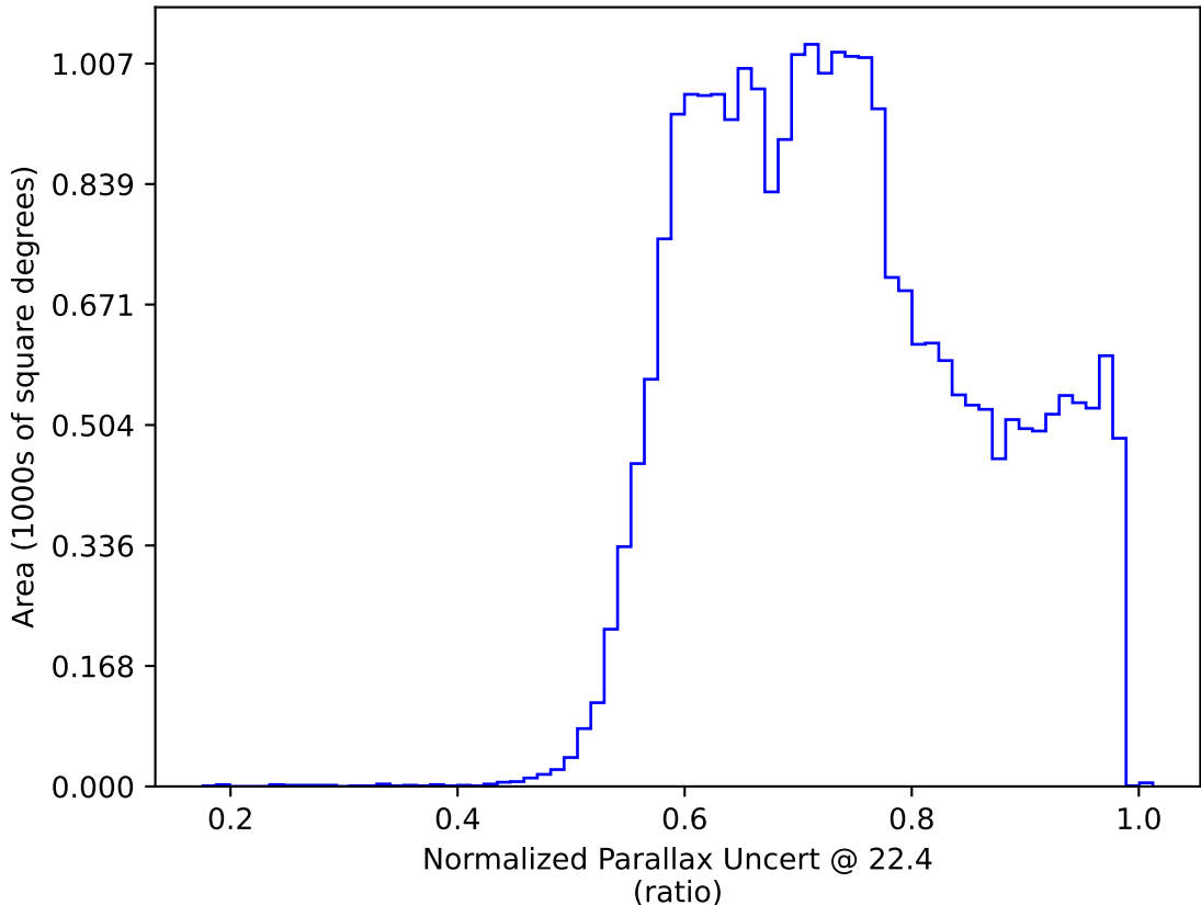
too_elab_heavy_r32_d2_griz_v3.4_10yrs : Normalized Parallax Uncert @ 22.4
