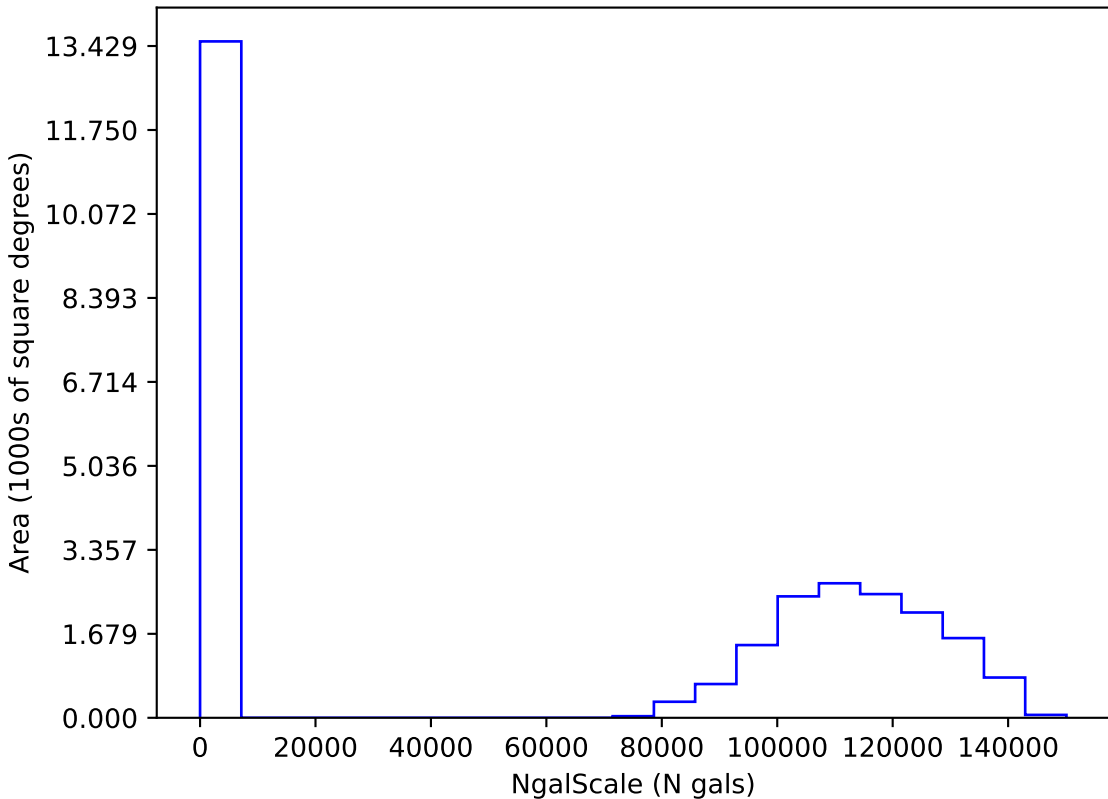
too_elab_heavy_r32_d2_griz_v3.4_10yrs i: NgalScale
