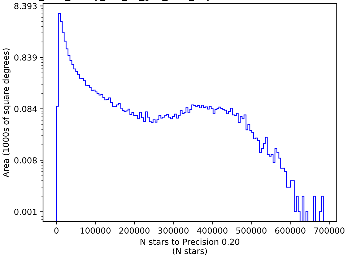
too_elab_heavy_r32_d2_griz_v3.4_10yrs z: N stars to Precision 0.20
