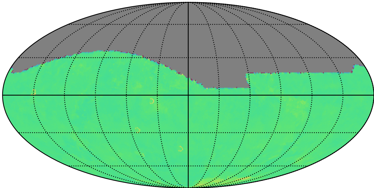
too_elab_heavy_r32_d2_griz_v3.4_10yrs r: Kuiper rotTelPos
