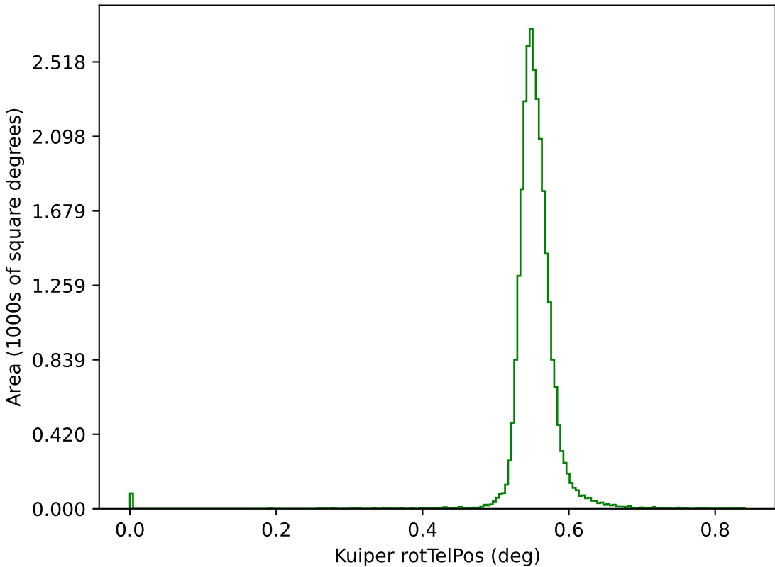
too_elab_heavy_r32_d2_griz_v3.4_10yrs g: Kuiper rotTelPos
