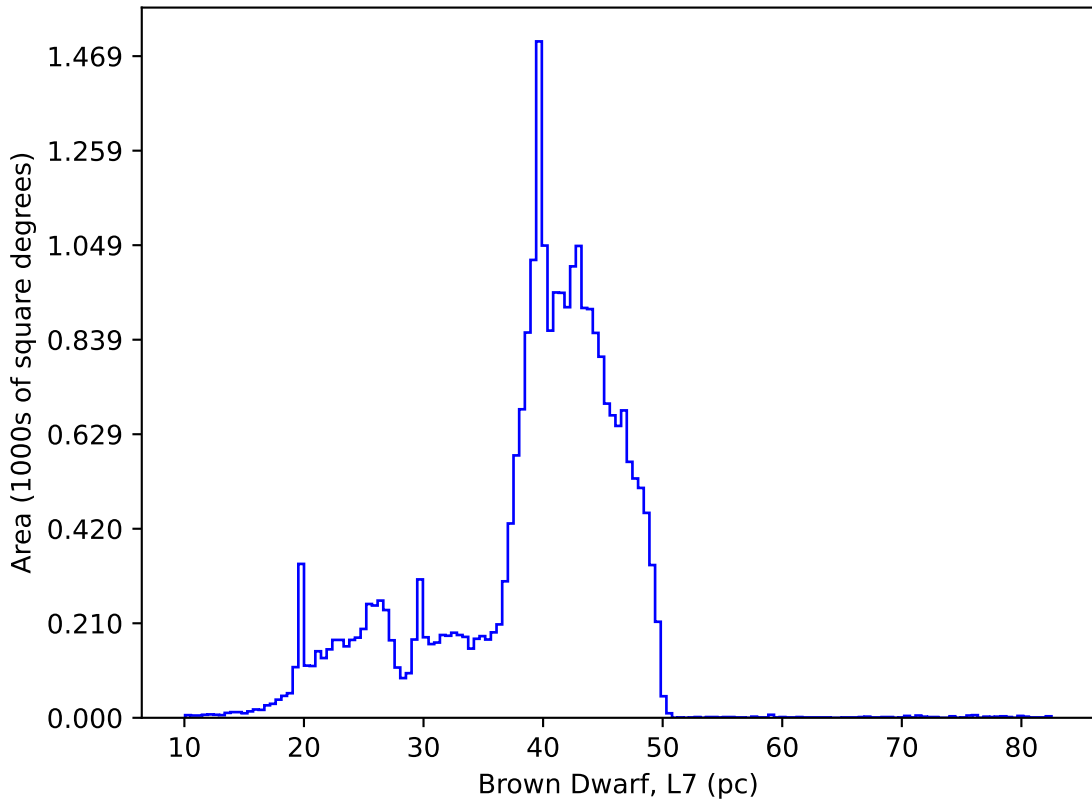
too_elab_heavy_r32_d2_griz_v3.4_10yrs : Brown Dwarf, L7
