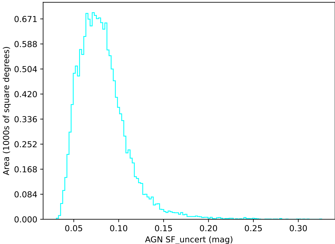
too_elab_heavy_r32_d2_griz_v3.4_10yrs u band: AGN SF_uncert
