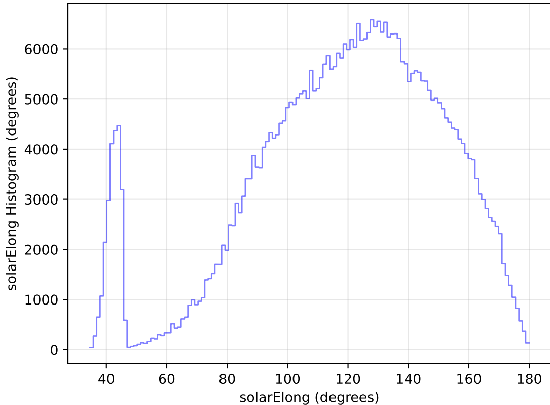
too_elab_heavy_r32_d2_griz_v3.4_10yrs WFD z band: solarElong Histogram
