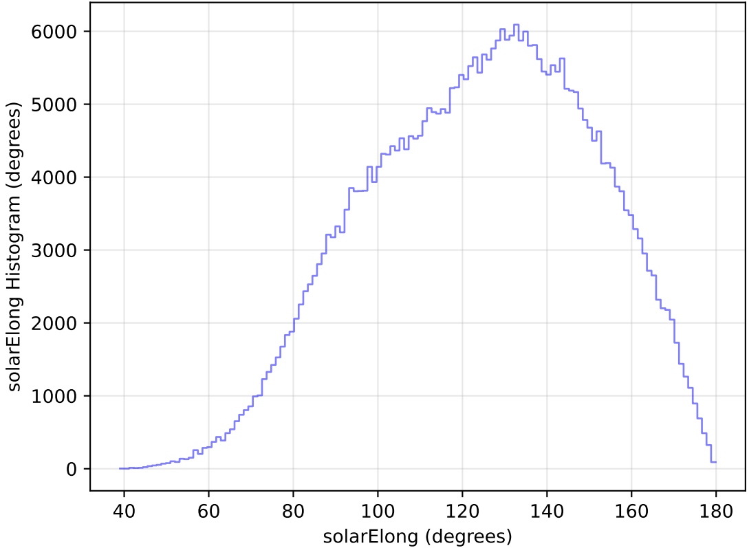
too_elab_heavy_r32_d2_griz_v3.4_10yrs WFD y band: solarElong Histogram
