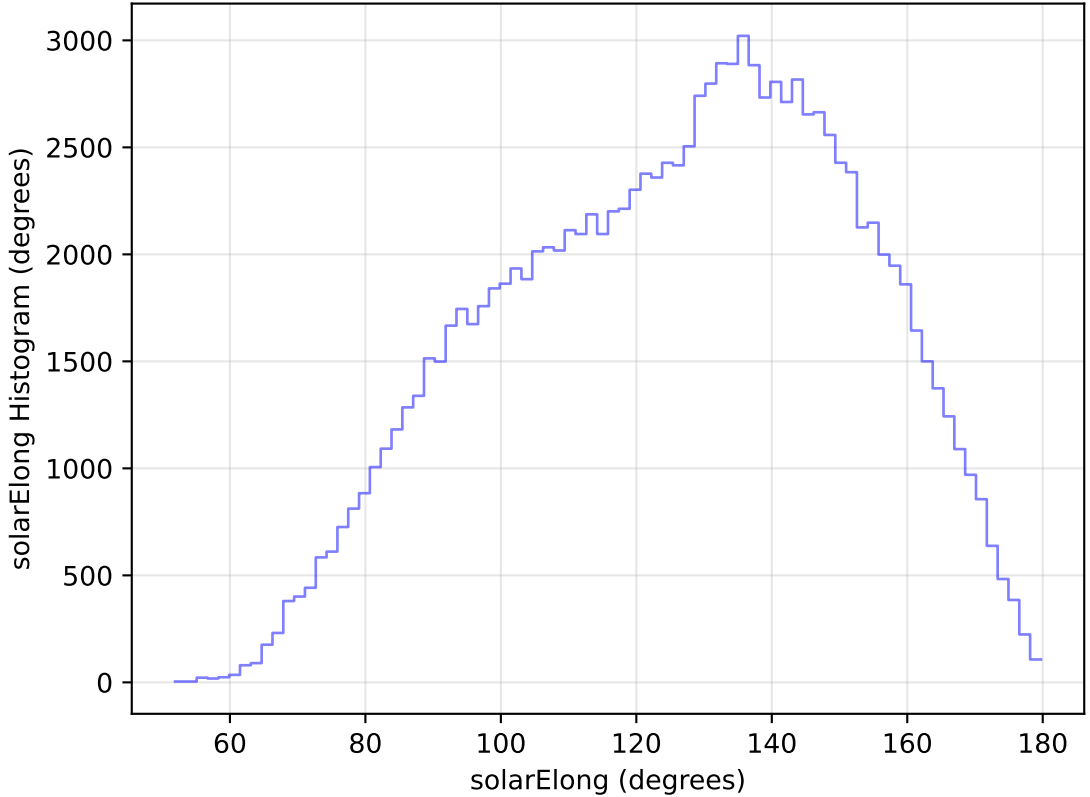
too_elab_heavy_r32_d2_griz_v3.4_10yrs WFD u band: solarElong Histogram
