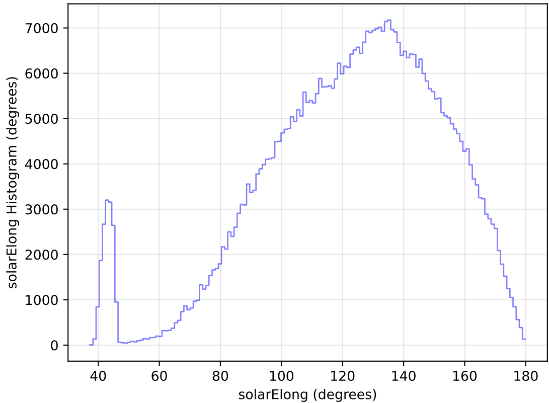
too_elab_heavy_r32_d2_griz_v3.4_10yrs WFD r band: solarElong Histogram
