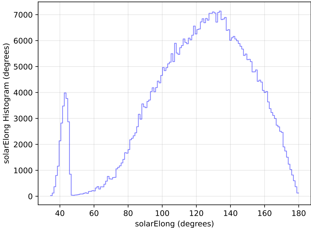
too_elab_heavy_r32_d2_griz_v3.4_10yrs WFD i band: solarElong Histogram
