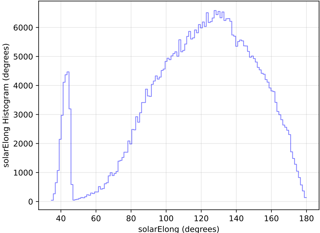
too_elab_heavy_r32_d2_griz_v3.4_10yrs All sky z band: solarElong Histogram
