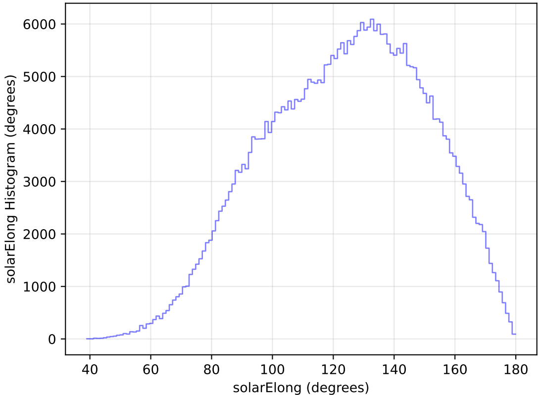
too_elab_heavy_r32_d2_griz_v3.4_10yrs All sky y band: solarElong Histogram
