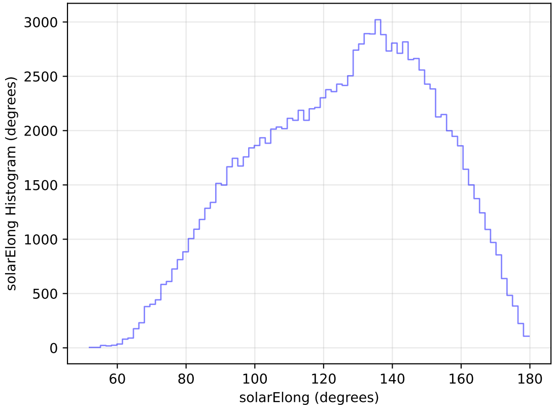
too_elab_heavy_r32_d2_griz_v3.4_10yrs All sky u band: solarElong Histogram
