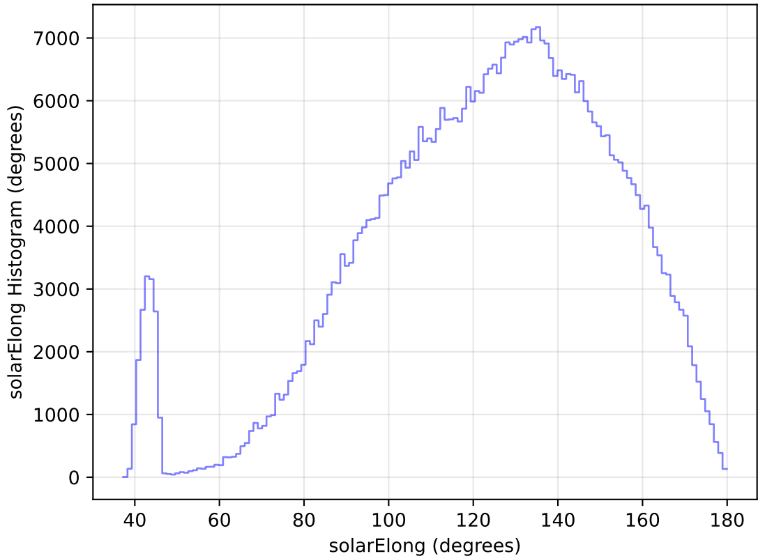
too_elab_heavy_r32_d2_griz_v3.4_10yrs All sky r band: solarElong Histogram
