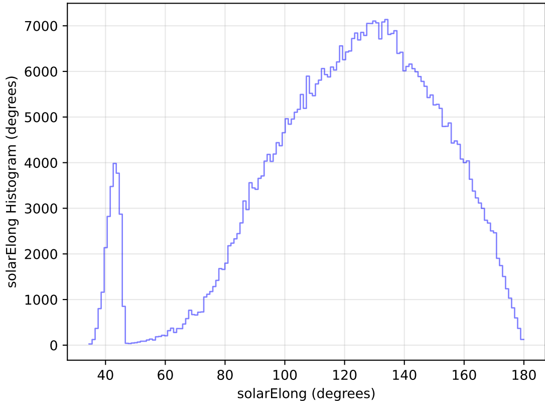
too_elab_heavy_r32_d2_griz_v3.4_10yrs All sky i band: solarElong Histogram
