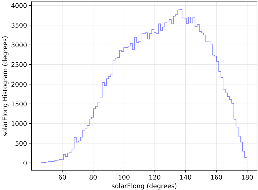
too_elab_heavy_r32_d2_griz_v3.4_10yrs All sky g band: solarElong Histogram
