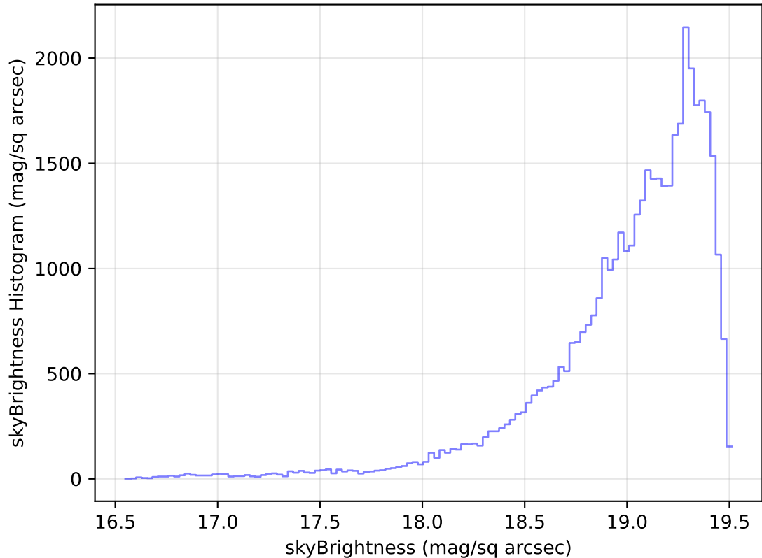
too_elab_heavy_r32_d2_griz_v3.4_10yrs Yr 1 z band: skyBrightness Histogram
