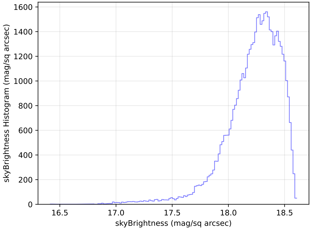
too_elab_heavy_r32_d2_griz_v3.4_10yrs Yr 1 y band: skyBrightness Histogram
