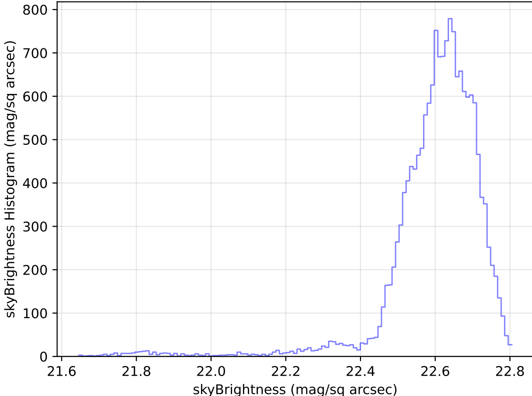
too_elab_heavy_r32_d2_griz_v3.4_10yrs Yr 1 u band: skyBrightness Histogram
