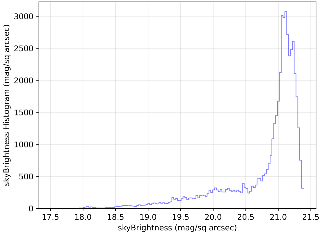
too_elab_heavy_r32_d2_griz_v3.4_10yrs Yr 1 r band: skyBrightness Histogram
