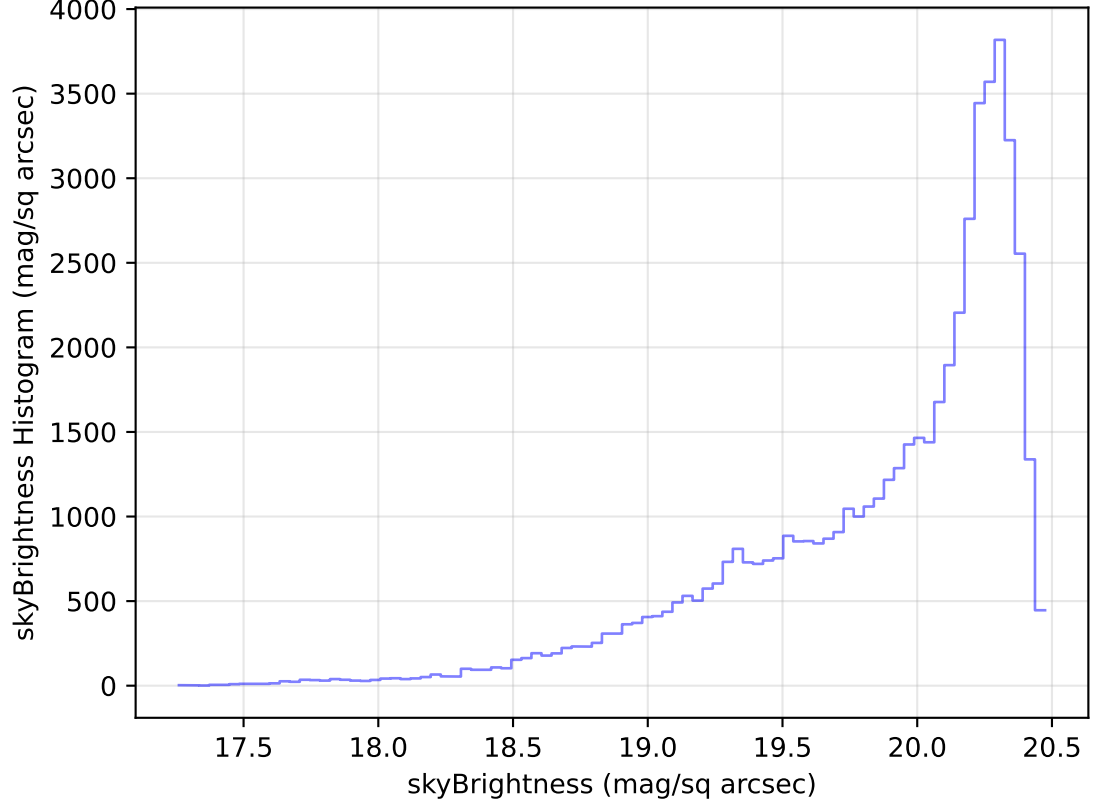
too_elab_heavy_r32_d2_griz_v3.4_10yrs Yr 1 i band: skyBrightness Histogram
