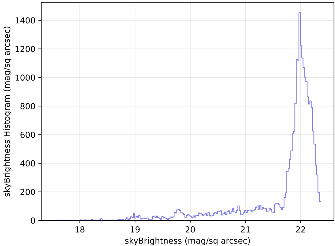
too_elab_heavy_r32_d2_griz_v3.4_10yrs Yr 1 g band: skyBrightness Histogram
