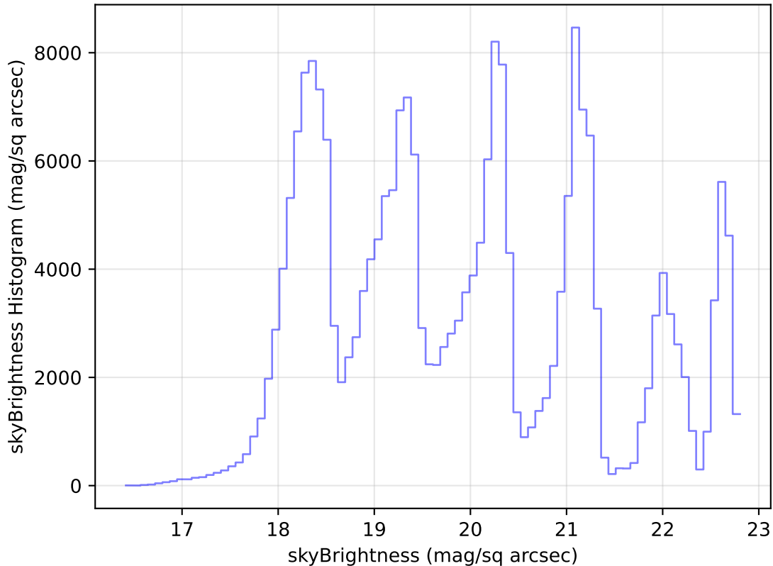
too_elab_heavy_r32_d2_griz_v3.4_10yrs Yr 1 all bands: skyBrightness Histogram
