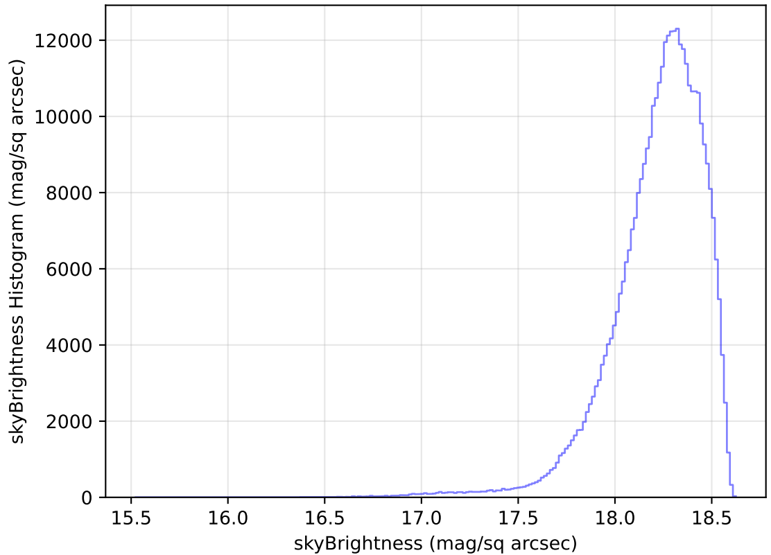
too_elab_heavy_r32_d2_griz_v3.4_10yrs WFD y band: skyBrightness Histogram
