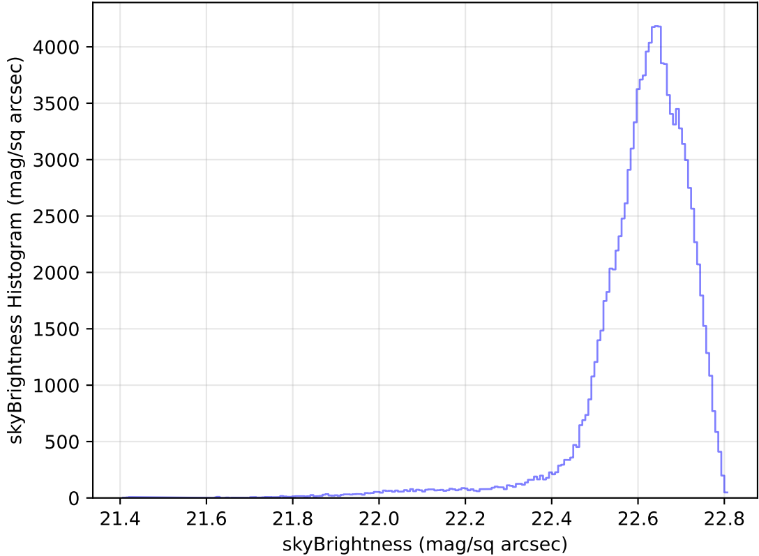
too_elab_heavy_r32_d2_griz_v3.4_10yrs WFD u band: skyBrightness Histogram
