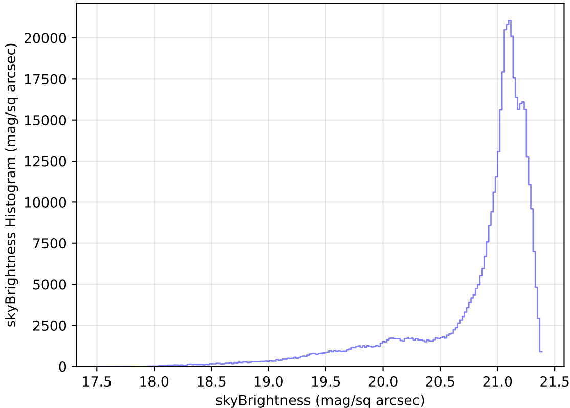
too_elab_heavy_r32_d2_griz_v3.4_10yrs WFD r band: skyBrightness Histogram
