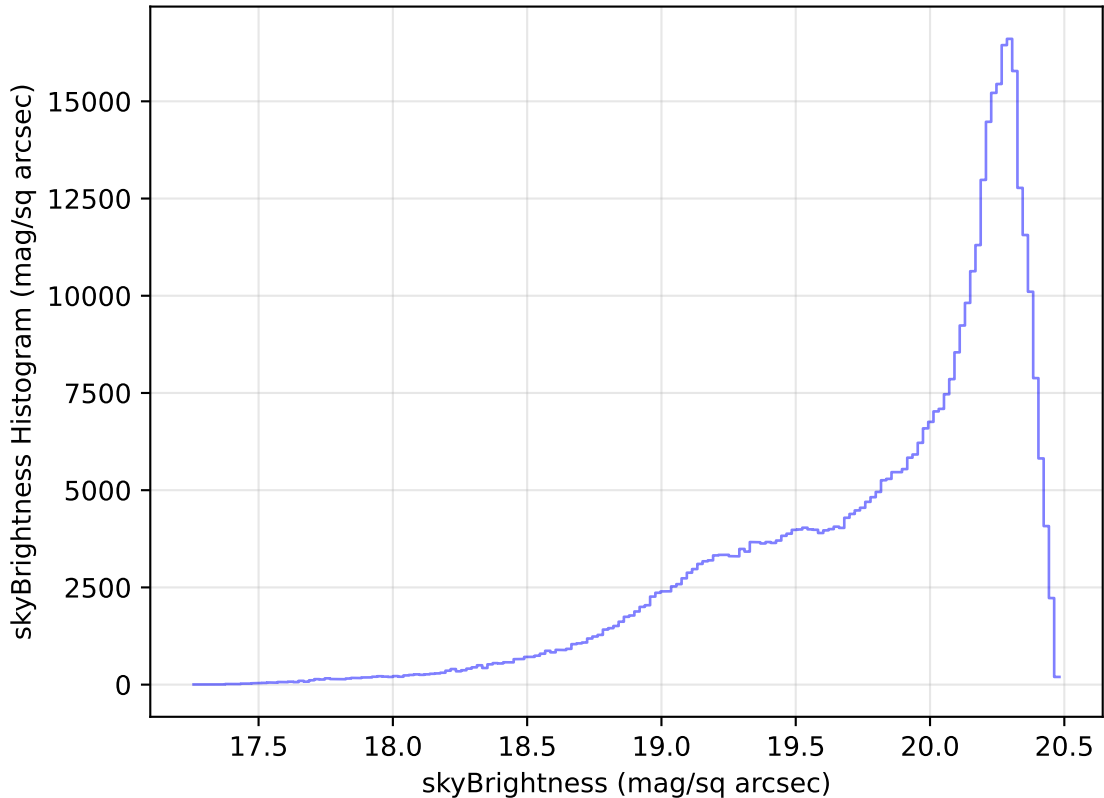
too_elab_heavy_r32_d2_griz_v3.4_10yrs WFD i band: skyBrightness Histogram
