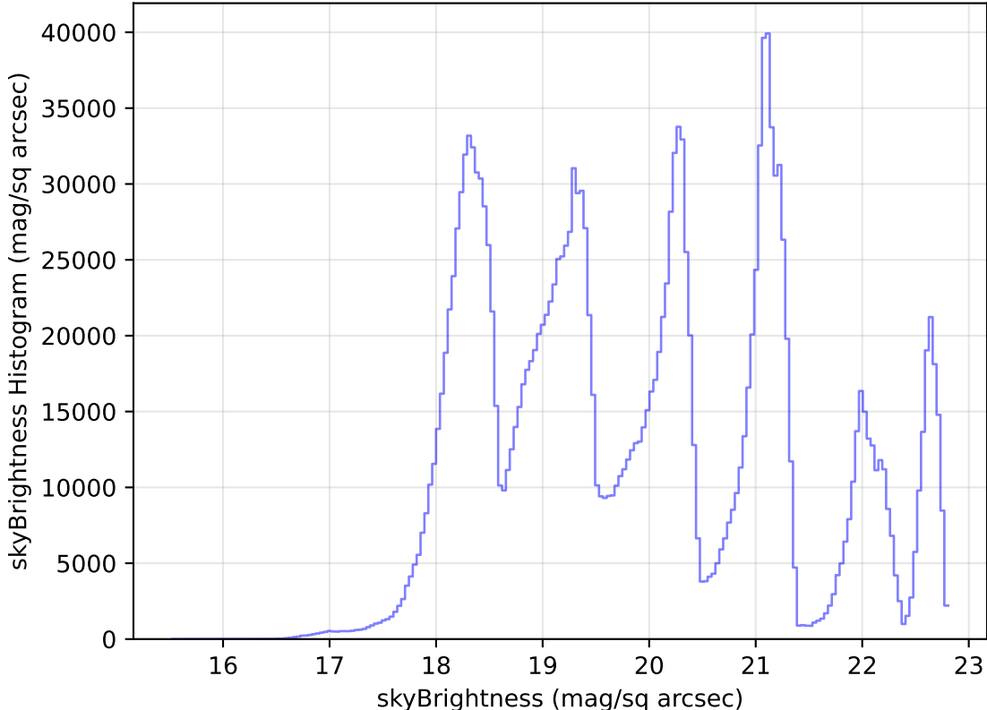
too_elab_heavy_r32_d2_griz_v3.4_10yrs WFD all bands: skyBrightness Histogram
