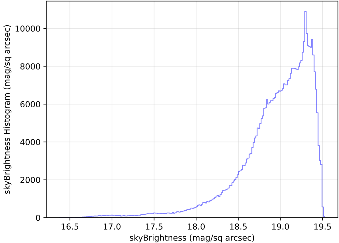
too_elab_heavy_r32_d2_griz_v3.4_10yrs All sky z band: skyBrightness Histogram
