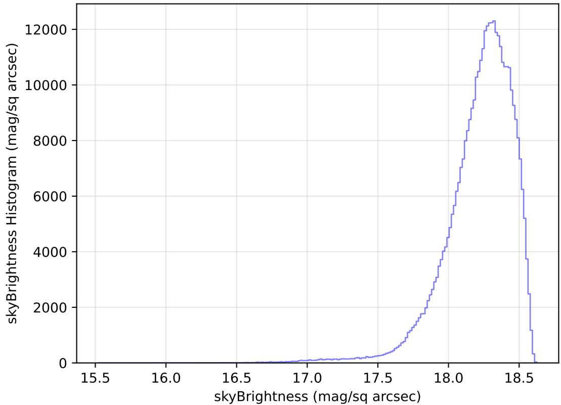
too_elab_heavy_r32_d2_griz_v3.4_10yrs All sky y band: skyBrightness Histogram
