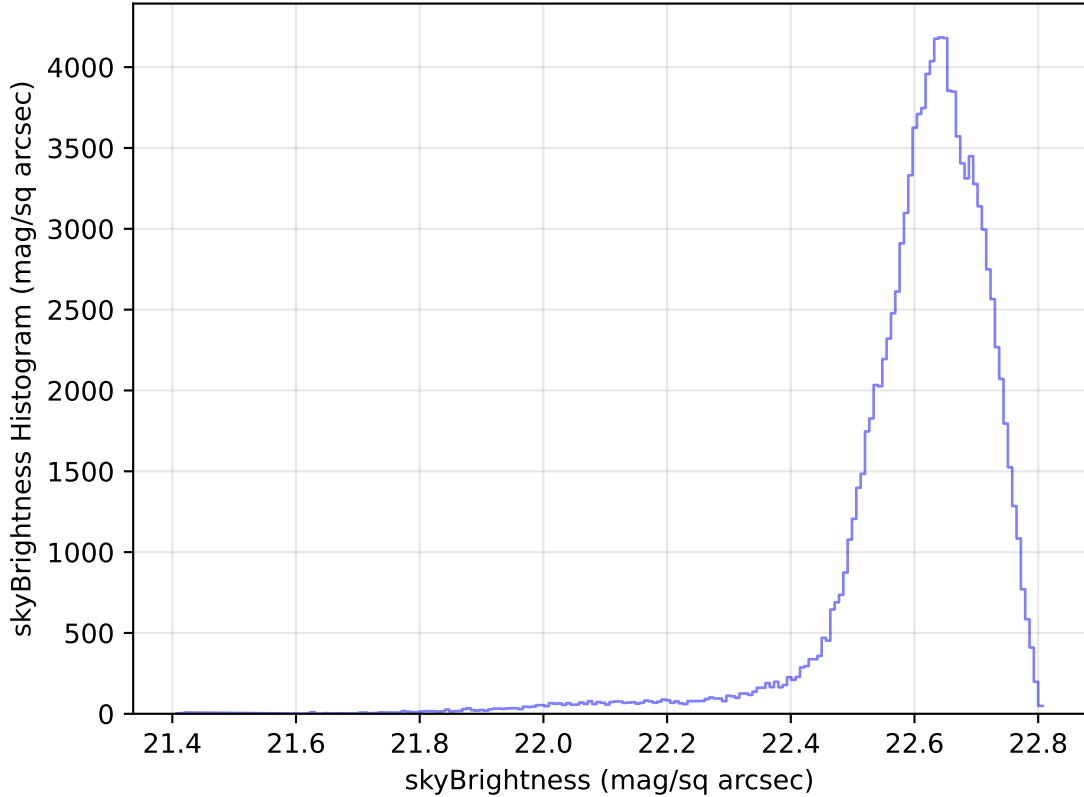
too_elab_heavy_r32_d2_griz_v3.4_10yrs All sky u band: skyBrightness Histogram
