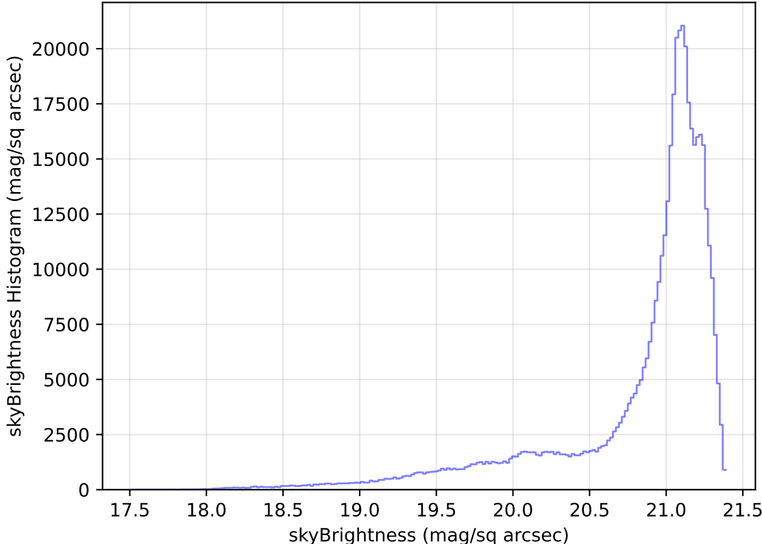
too_elab_heavy_r32_d2_griz_v3.4_10yrs All sky r band: skyBrightness Histogram
