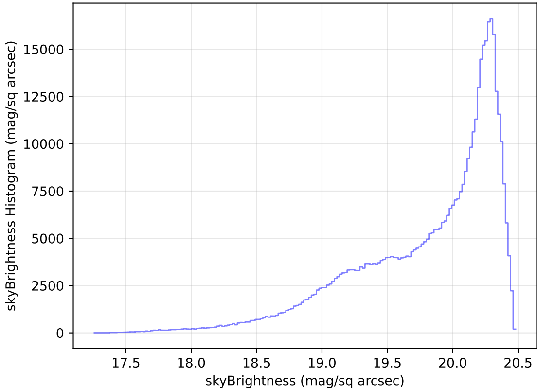
too_elab_heavy_r32_d2_griz_v3.4_10yrs All sky i band: skyBrightness Histogram
