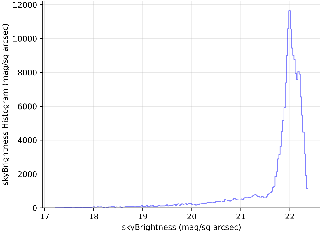
too_elab_heavy_r32_d2_griz_v3.4_10yrs All sky g band: skyBrightness Histogram
