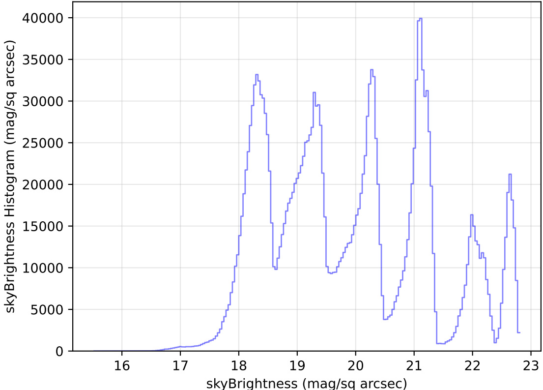
too_elab_heavy_r32_d2_griz_v3.4_10yrs All sky all bands: skyBrightness Histogram
