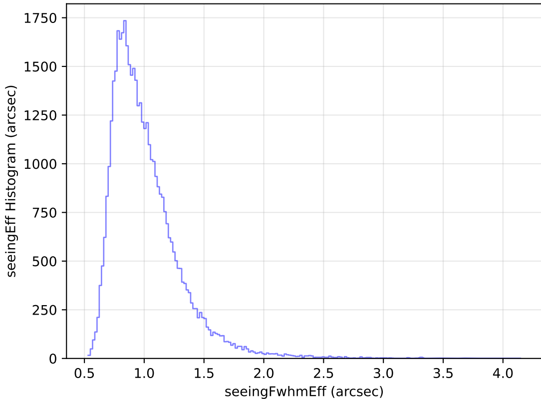
too_elab_heavy_r32_d2_griz_v3.4_10yrs Yr 1 z band: seeingEff Histogram
