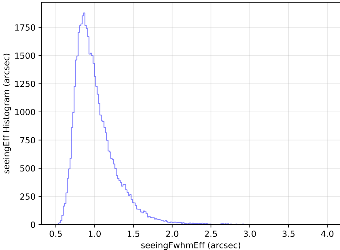
too_elab_heavy_r32_d2_griz_v3.4_10yrs Yr 1 y band: seeingEff Histogram
