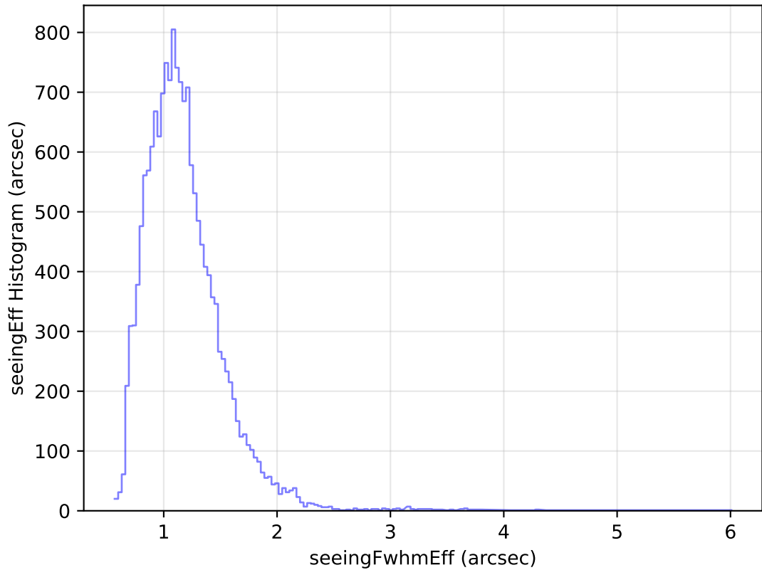
too_elab_heavy_r32_d2_griz_v3.4_10yrs Yr 1 u band: seeingEff Histogram
