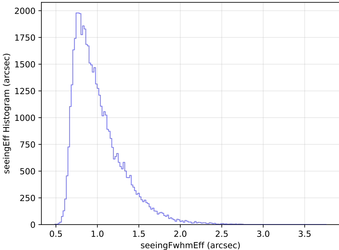
too_elab_heavy_r32_d2_griz_v3.4_10yrs Yr 1 r band: seeingEff Histogram
