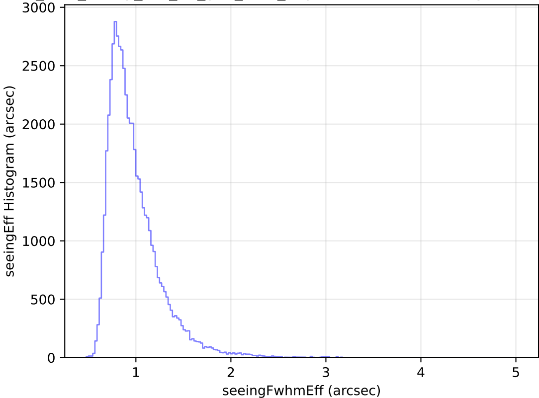
too_elab_heavy_r32_d2_griz_v3.4_10yrs Yr 1 i band: seeingEff Histogram
