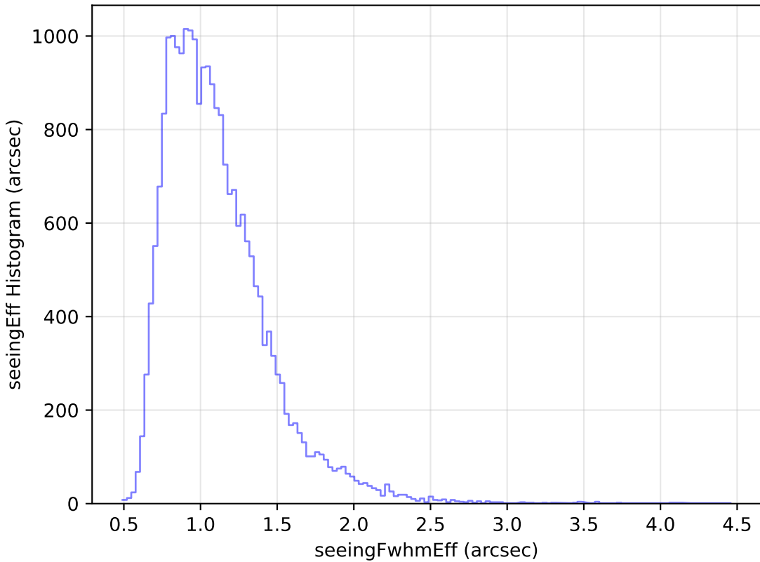
too_elab_heavy_r32_d2_griz_v3.4_10yrs Yr 1 g band: seeingEff Histogram
