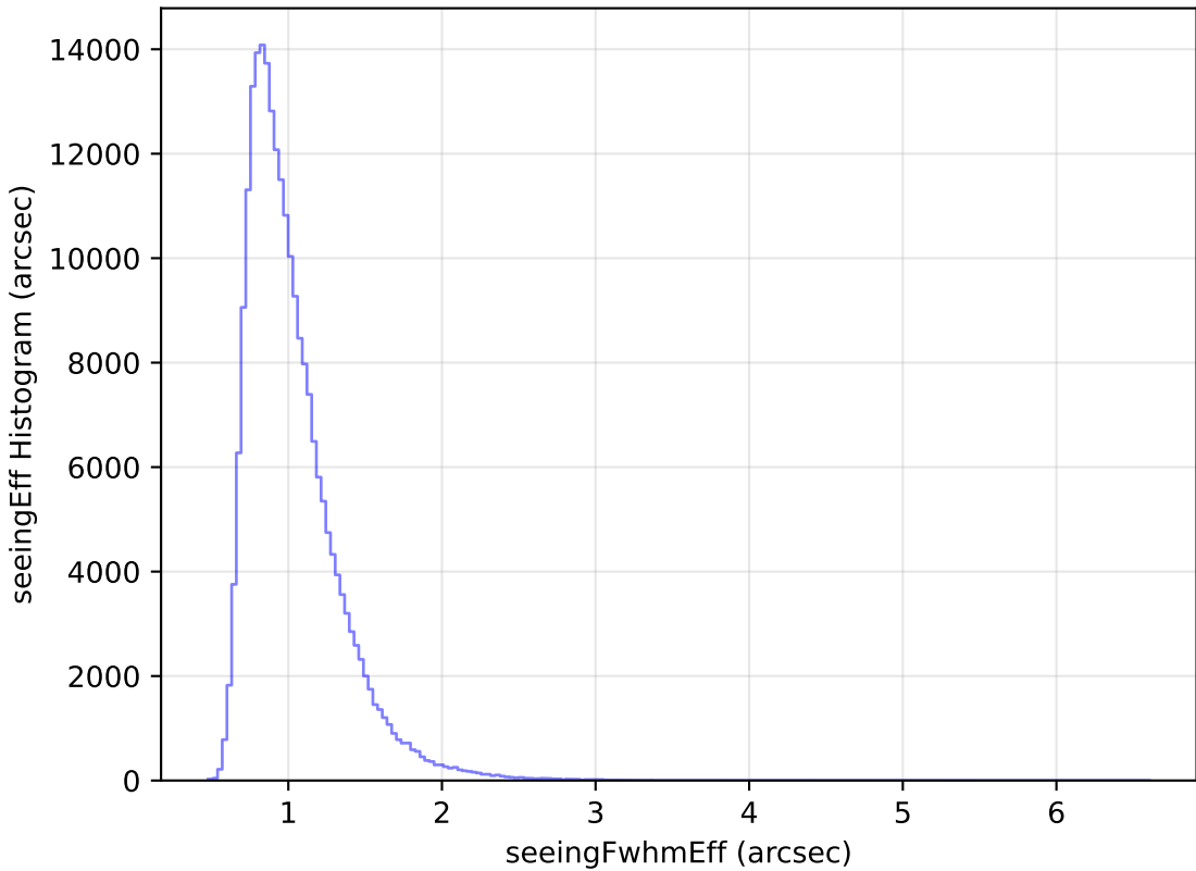
too_elab_heavy_r32_d2_griz_v3.4_10yrs Yr 1 all bands: seeingEff Histogram
