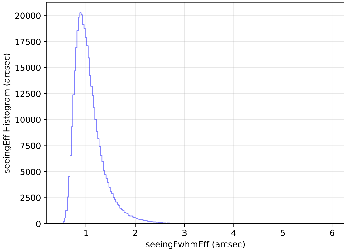
too_elab_heavy_r32_d2_griz_v3.4_10yrs WFD y band: seeingEff Histogram
