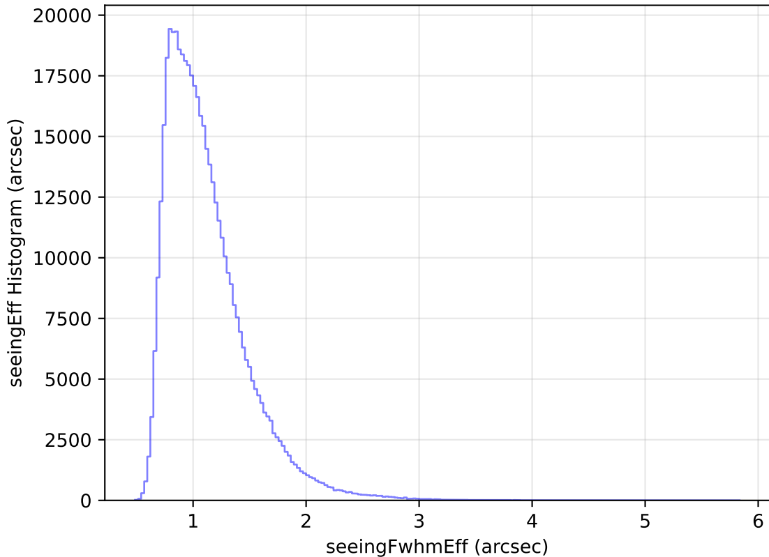
too_elab_heavy_r32_d2_griz_v3.4_10yrs WFD r band: seeingEff Histogram
