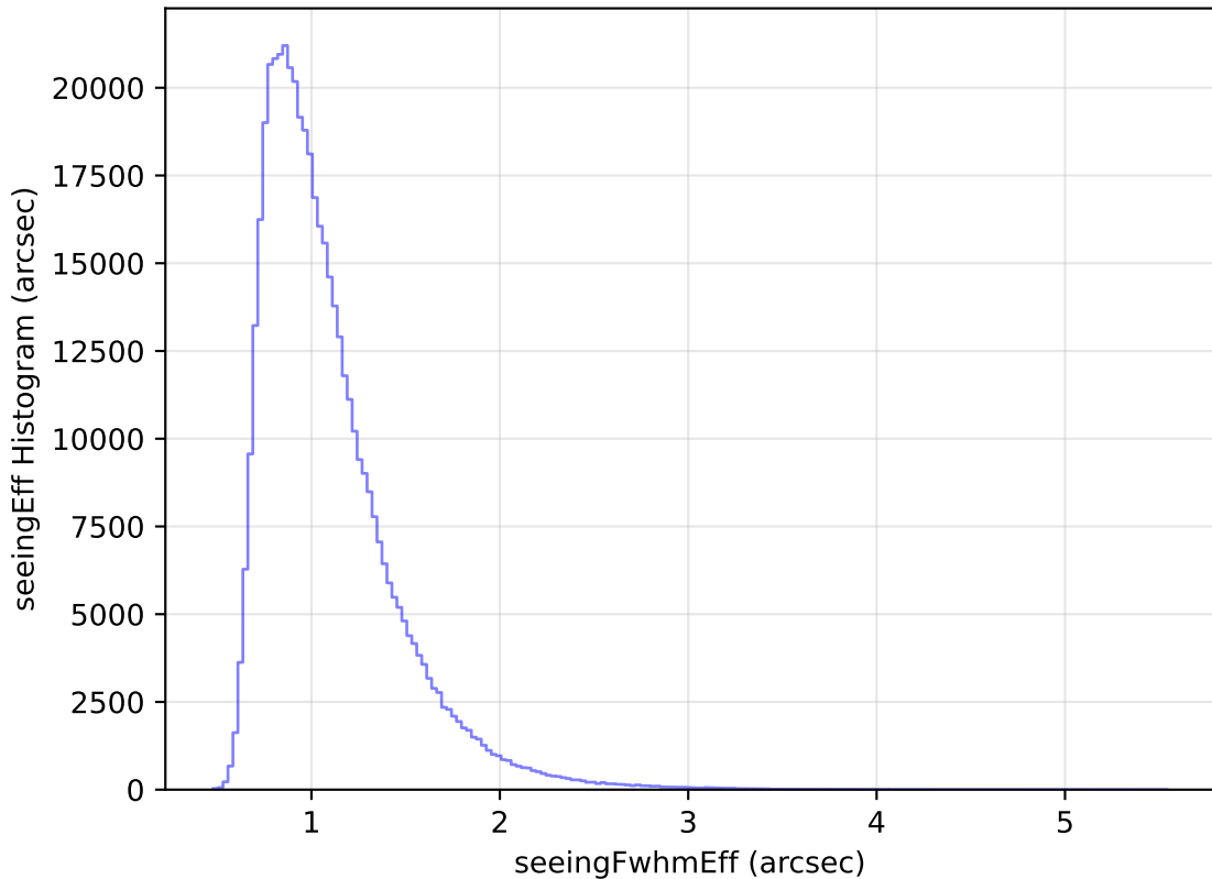
too_elab_heavy_r32_d2_griz_v3.4_10yrs WFD i band: seeingEff Histogram
